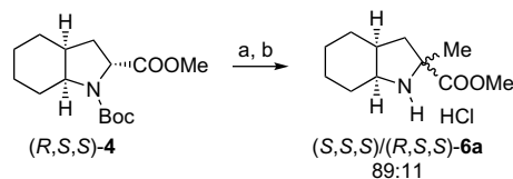
Scheme 5. \alpha -Methylation reaction of ( R,S,S )- 4 . Reagents and conditions: (a) LDA, MeI, THF, -78 to -50^\circ\text{C} ; (b) 3 N HCl/EtOAc, rt.
