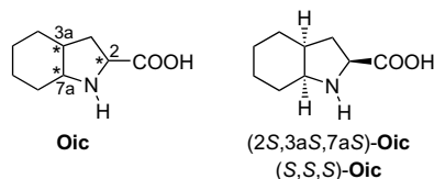
Figure 1. Structure of (2S,3aS,7aS)-octahydroindole-2-carboxylic acid.
