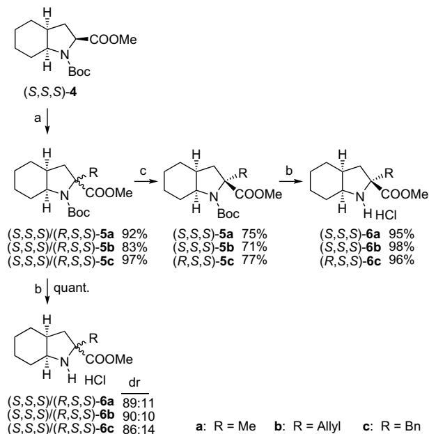
Scheme 3. \alpha -Alkylations of (S,S,S) -4. Reagents and conditions: (a) LDA, RX, THF, -78^\circ\text{C} ; (b) 3 N HCl/EtOAc, rt; (c) column chromatography of the diastereomeric mixtures ( \text{SiO}_2 , EtOAc/hexanes 1:10) furnishes pure (S,S,S) -5a, (S,S,S) -5b and (R,S,S) -5c. RX = MeI, AllylBr, BnBr.
