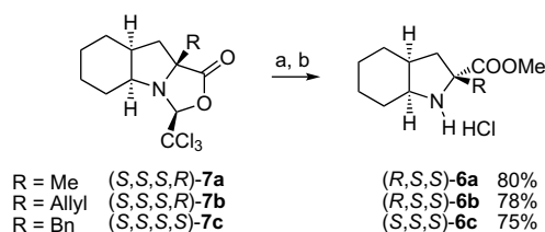
Scheme 4. Synthesis of enantiopure ( R,S,S )- 6a , ( R,S,S )- 6b and ( S,S,S )- 6c . Reagents and conditions: (a) MeONa, MeOH, rt; (b) \text{CH}_3\text{COCl} , MeOH, reflux.
