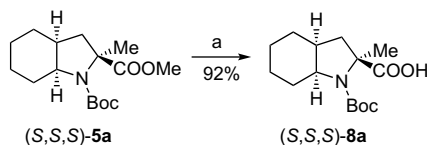
Scheme 6. Synthesis of enantiopure (S,S,S)- 8a . Reagents and conditions: (a) 1 N KOH, MeOH/H 2 O, reflux.
