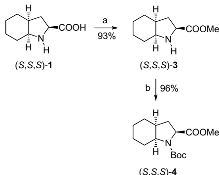
Scheme 2. Synthesis of enantiopure (S,S,S) -4. Reagents and conditions: (a) \text{SOCl}_2 , MeOH, rt; (b) \text{Boc}_2\text{O} , i - \text{Pr}_2\text{EtN} , 4-dimethylaminopyridine, THF, rt.
