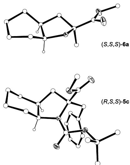
Figure 2. X-ray crystal structures of ( S,S,S )- 6a (the chlorine atom is not shown) and ( R,S,S )- 5c . Heteroatoms are drawn as thermal ellipsoids. Most hydrogens have been omitted for clarity.
