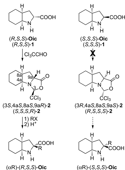
Scheme 1. Reported synthesis for \alpha -alkyl derivatives of (R,S,S) -Oic (Ref. 10a).
